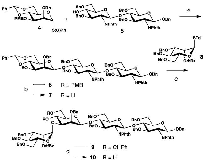
Scheme 1. Synthesis of Tetrasaccharide 10 a
