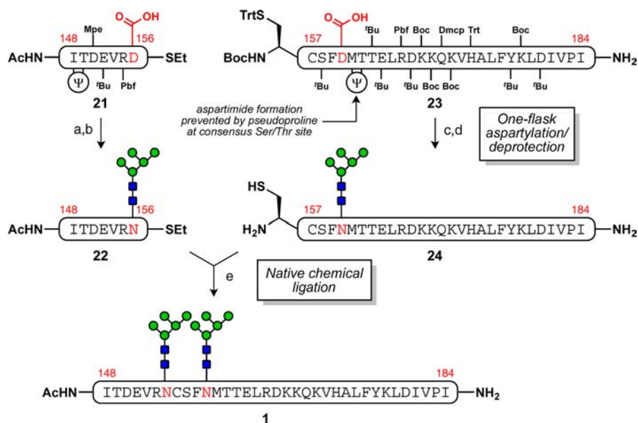
Scheme 5. Synthesis of V1V2 Glycopeptide 1 a
