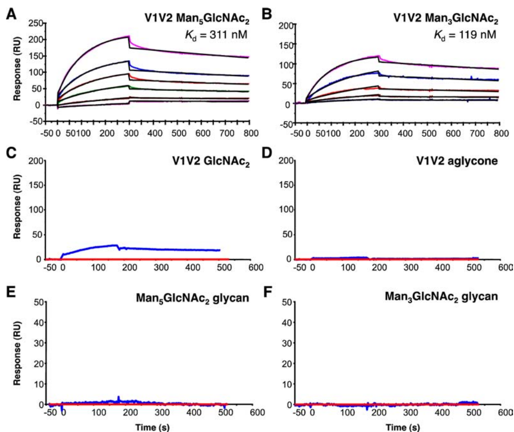
Figure 2. Binding of mAb PG9 to gp120 V1V2 glycopeptides. SPR sensorgrams showing binding of mAb PG9 to V1V2 glycopeptides derivatized with \text{Man}_5\text{GlcNAc}_2 (A) and \text{Man}_3\text{GlcNAc}_2 (B). V1V2 \text{Man}_5\text{GlcNAc}_2 binding curves are shown for glycopeptide concentrations at 5, 10, 20, 30, and 40 \mu\text{g}/\text{mL} and V1V2 \text{Man}_3\text{GlcNAc}_2 at 1, 2, 5, 10, and 20 \mu\text{g}/\text{mL} . Control SPR sensorgrams showing minimal to no binding of mAb PG9 to V1V2 \text{GlcNAc}_2 (C), V1V2 aglycone (D), \text{Man}_5\text{GlcNAc}_2 glycan alone (E), and \text{Man}_3\text{GlcNAc}_2 glycan alone (F). V1V2 \text{GlcNAc}_2 and aglycone peptides were injected at 200 \mu\text{g}/\text{mL} (C, D) and \text{Man}_5\text{GlcNAc}_2 and \text{Man}_3\text{GlcNAc}_2 glycans at 25 \mu\text{g}/\text{mL} (E, F) over PG9 captured on anti-human IgG (Fc-specific) surfaces. SPR data were derived following subtraction of a nonspecific signal on a control anti-RSV mAb (Synagis, red curve in panels C–F).
