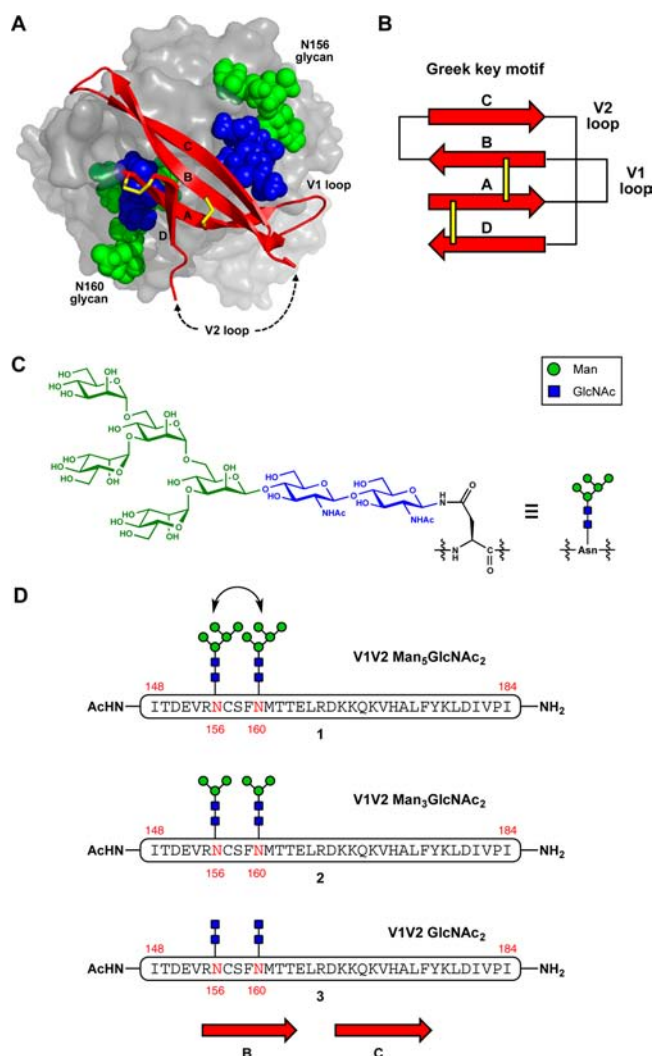
Figure 1. Design of gp120 V1V2 domain broadly neutralizing epitope mimics. (A) Crystal structure of a scaffolded V1V2 domain from the CAP45 strain of HIV-1 (red ribbons) in complex with PG9 Fab (gray surface) (PDB ID 3U4E with scaffold hidden). The glycans at N160 and N156 are depicted with colored spheres representing atoms of the mannose (green) and N -acetylglucosamine (blue) residues. Disulfide bonds are shown as yellow sticks. Dashed arrows indicate where the disordered region of the V2 loop would be connected. The figure was created using PyMOL. (B) Schematic of the Greek key topology of the V1V2 domain. Strands are represented as arrows and disulfide bonds as yellow bars. (C) Chemical structure of \text{Man}_5\text{GlcNAc}_2\text{-Asn} . (D) Structures of candidate BnAb antigens, derived from residues 148–184 of the A244 strain gp120 (HXB2 numbering), encompassing the B and C \beta -strands (approximate location shown with red arrows) of the V1V2 domain, and bearing two N -linked \text{Man}_5\text{GlcNAc}_2 , \text{Man}_3\text{GlcNAc}_2 , or \text{GlcNAc}_2 oligosaccharides.
