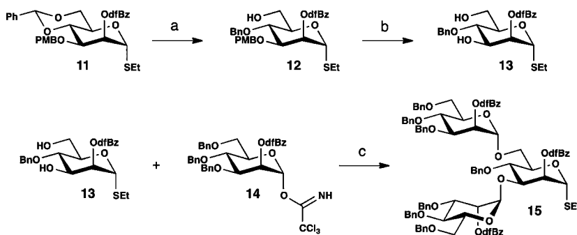
Scheme 2. Synthesis of Trisaccharide Donor 15 a
