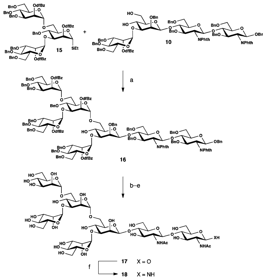
Scheme 3. Synthesis of Heptasaccharide 18 a
