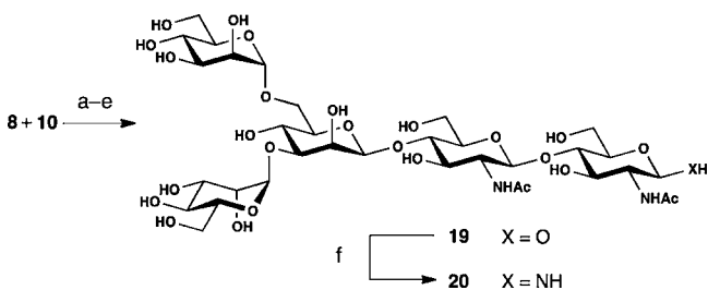
Scheme 4. Synthesis of Pentasaccharide 20 a
